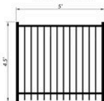
Model:C01-A-G4.5X5 Flat Top 2 Rail Gate 4.5'x5'
