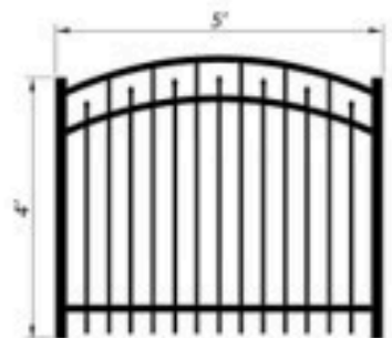
Mode: C06-A-AG4x5 Arched 3 rail Gate 4'x5'
