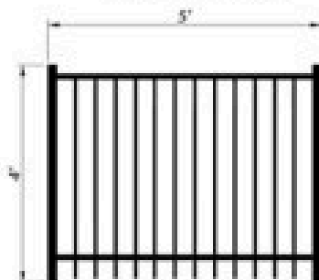
Model: C01-A-G4X5 Flat Top 2 Rail Gate 4'x5'
